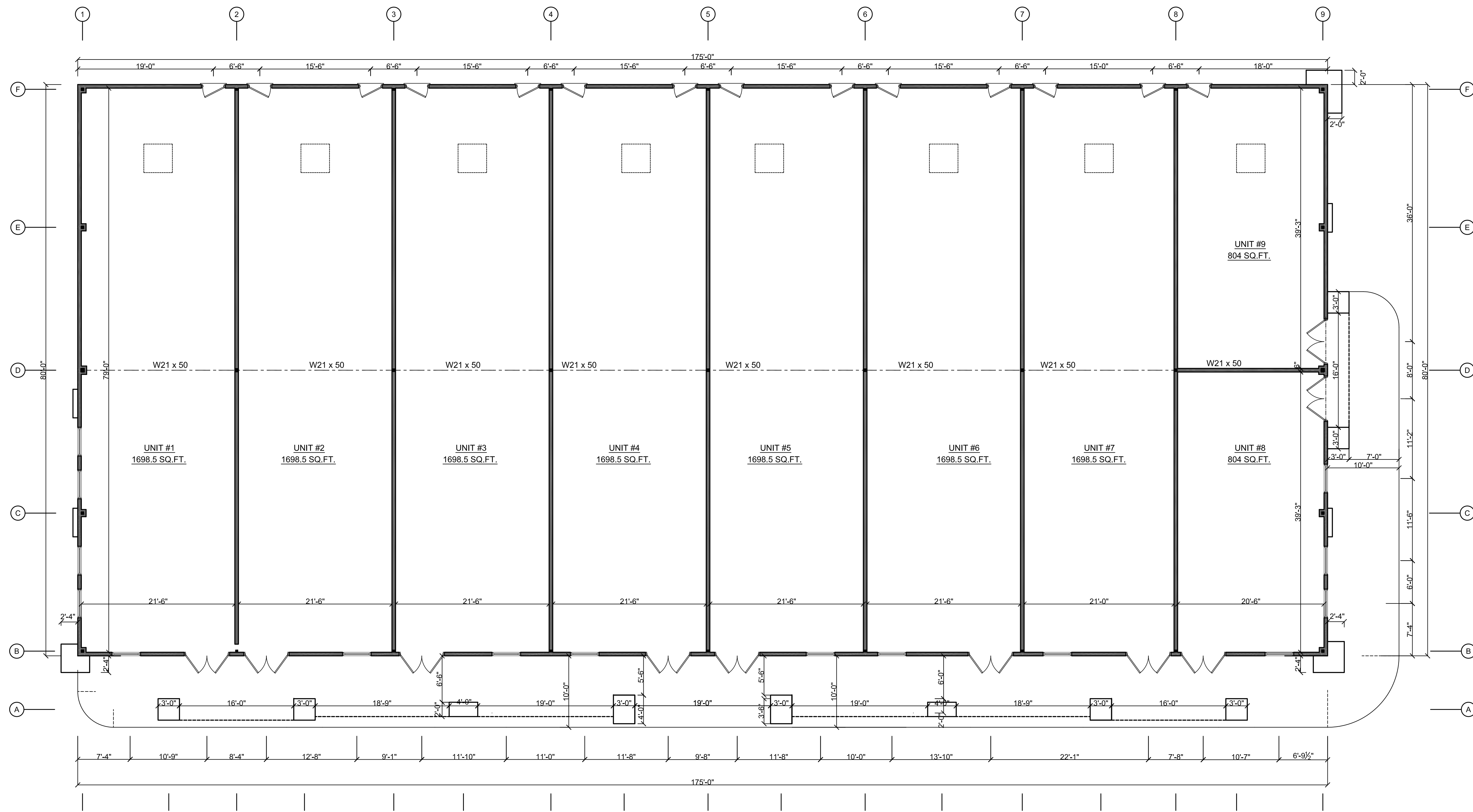
1 FLOOR PLAN 1/8" = 1'-0"
